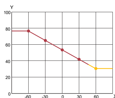
Example of five point temperature curve. Y-axis: Setpoint [°C]. X-axis: Outdoor temperature [°C].
