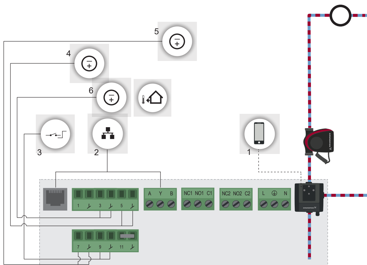
Example of MIXIT in a combined heating and cooling system
