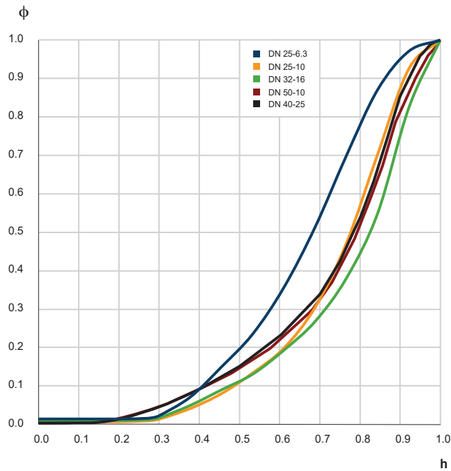
Inherent flow characteristic for A-AB in modified equal percentage. X-axis: Relative travel, h . Y-axis: Relative flow coefficient, \Phi .
