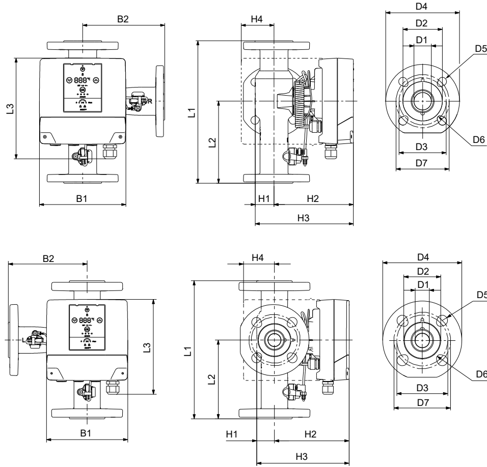
Dimensions [mm]
