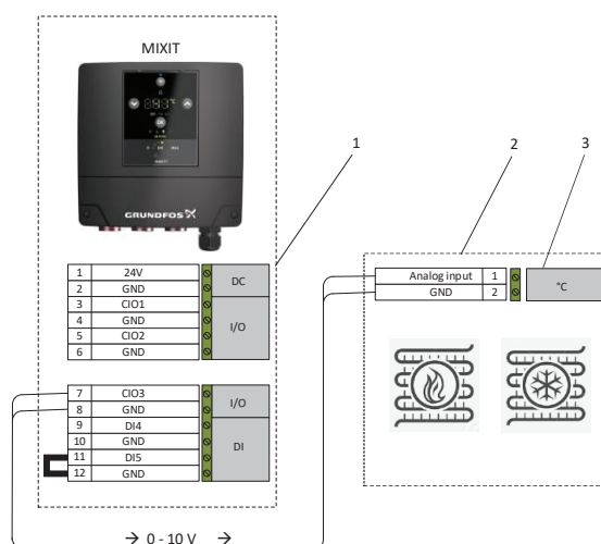
Supply source setpoint configuration of one MIXIT unit
