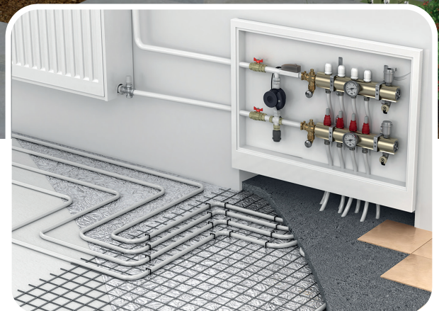
Suelo radiante / Underfloor heating
