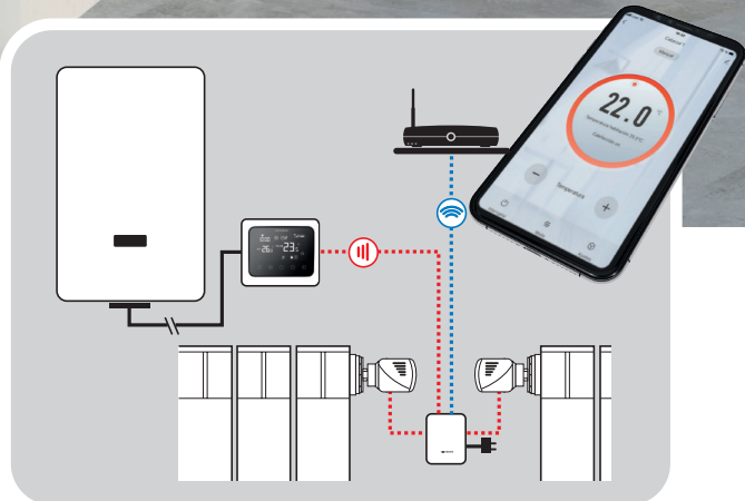
GE-Smart Wifi
